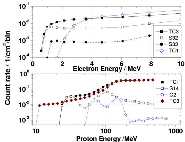
Fig. 2. Proton and electron responses shown for selected scalers as a function of incoming particle energy
