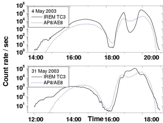
Fig. 6. Comparison of the measured and computed (NASA AP8/AE8 static models) belt profiles for a quiet and post solar event radiation environment
