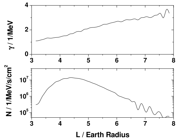
Fig. 4. Electron spectral parameters N and \gamma shown as a function of the L -parameter inside of the radiation belt
