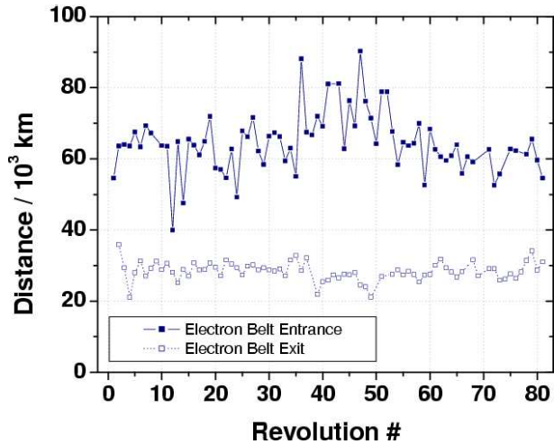
Fig. 5. Position of the electron belt entry and exit regions as a function of the INTEGRAL orbit number
