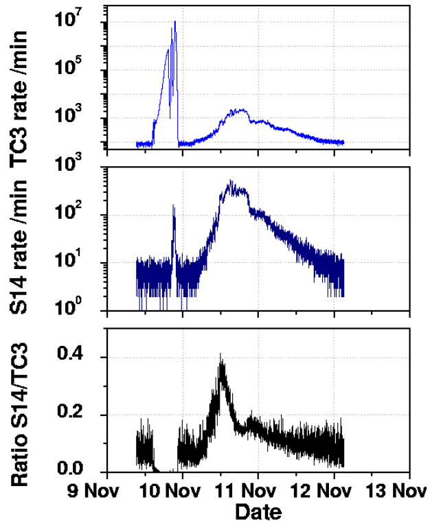
Fig. 7. Particle rates and rates ratio for two scalers with the large solar event of revolution 9 (right peak)
