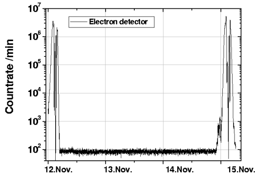
Fig. 3. Typical IREM count rate along the spacecraft orbit measured by the electron detector TC3
